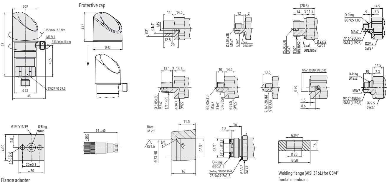
Flange adapter
